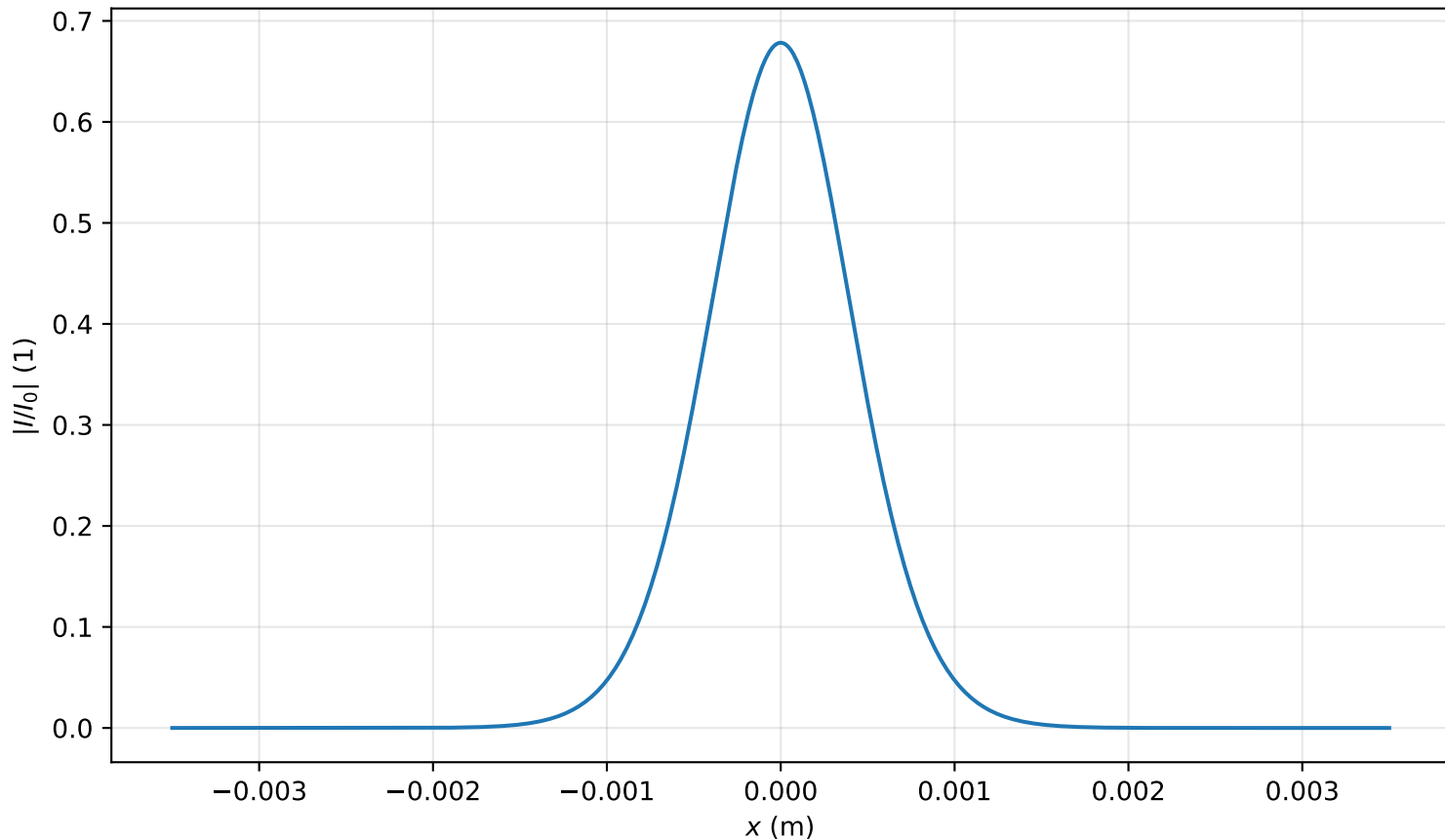
Intensity profile I(x, y = 0, z = 1.911m)/I_0 , P_{in}=0.3P_{cr} , artificial time
